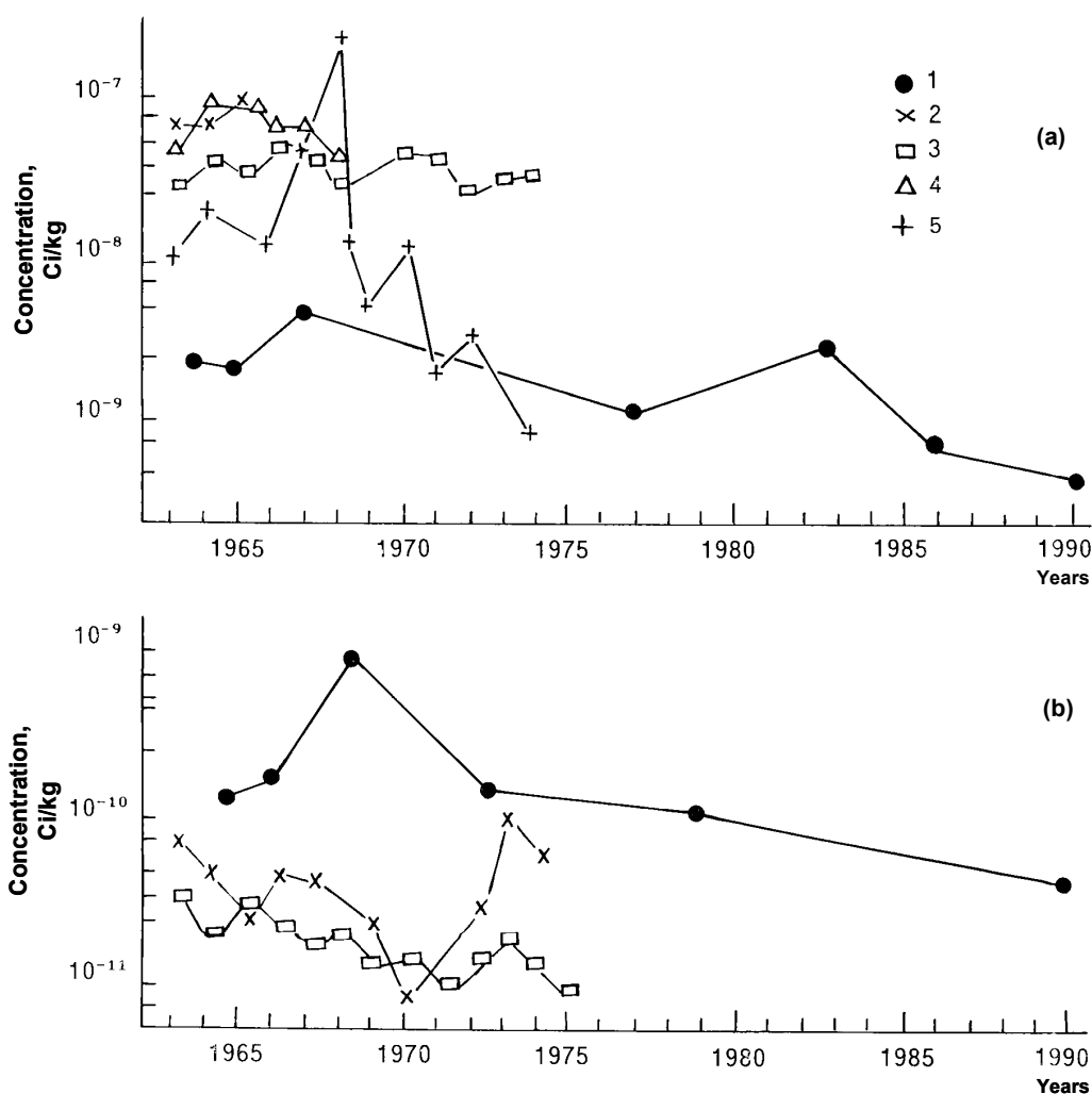
FIG. 14. Cesium-137 concentrations.
