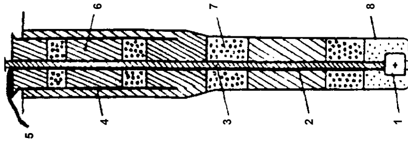
FIG. 17. Underground tests in a vertical shaft (borehole).
